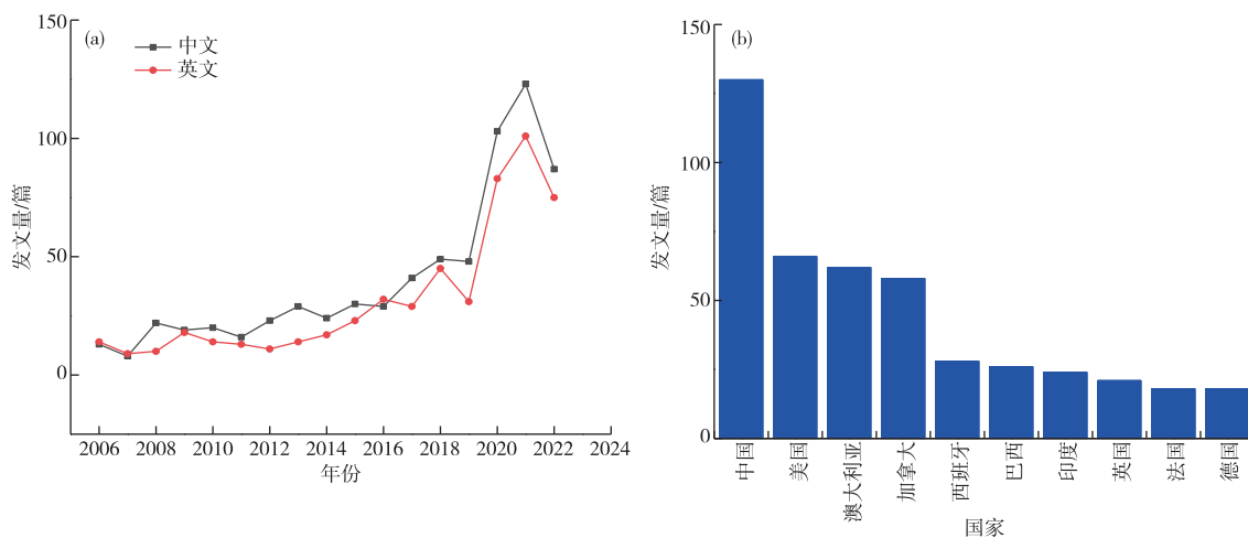
图1 2006—2022年矿区场地污染阻隔及生态修复技术领域年度发文量(a)及发文国家与地区(b) Fig. 1 Annual publication volume(a)and the countries and regions publishing articles(b) in the field of pollution control, barrier technologies, and ecological restoration techniques for mining area sites from 2006 to 2022
